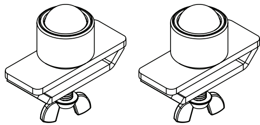
436BT — Steel 436BTS — Stainless Steel BALL TRANSFER HEAD ATTACHMENT SET
